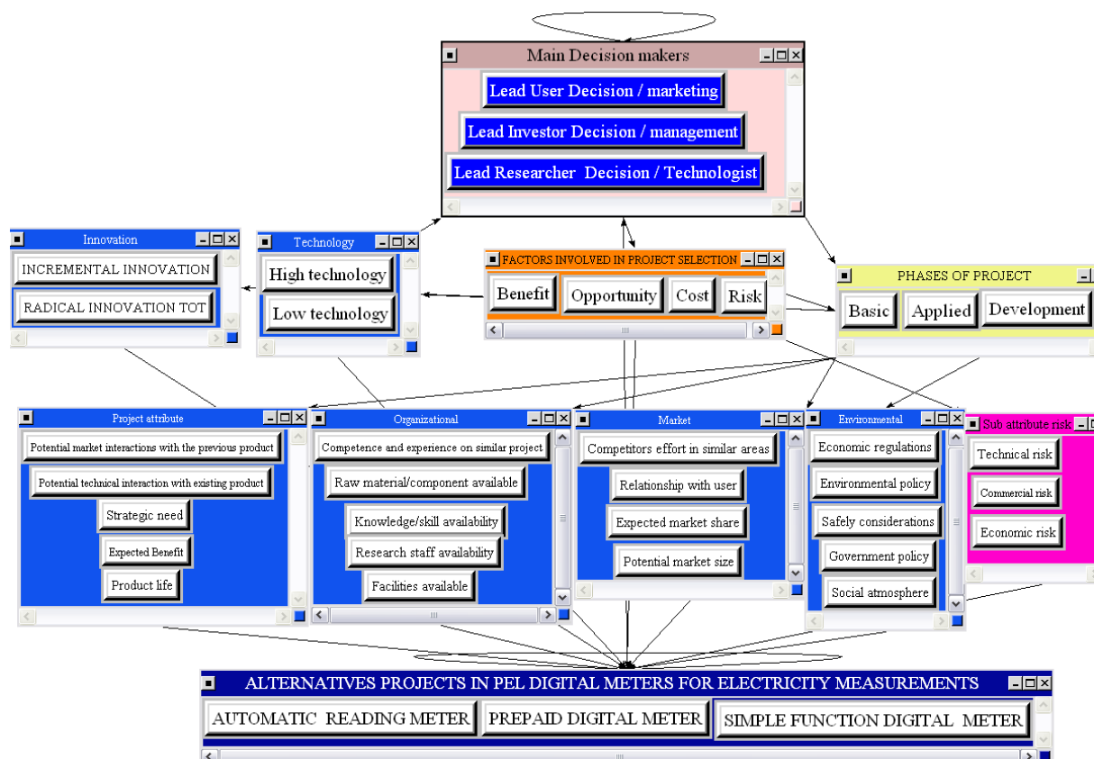
Figure 1. Analytic network framework showing the various attributes of project selection
